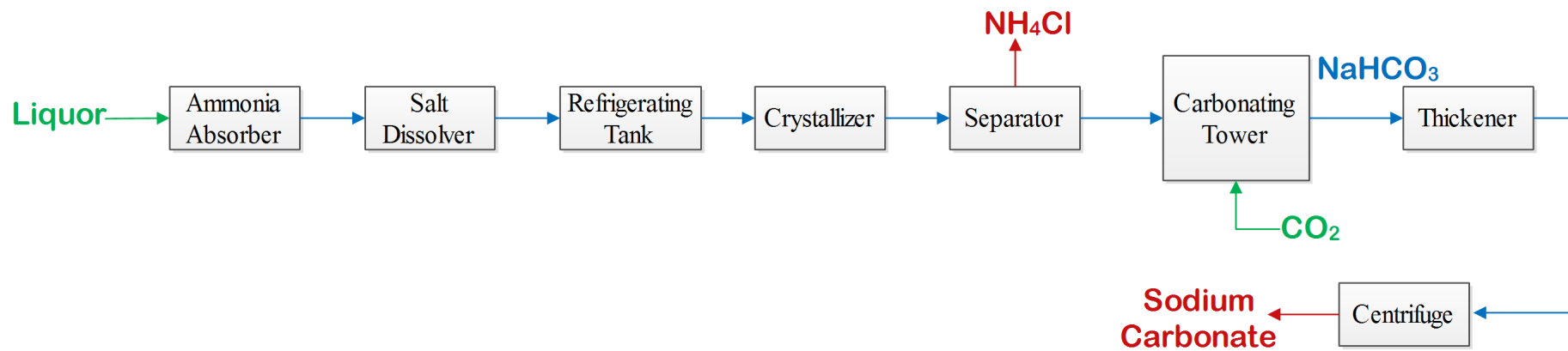
Figure: Manufacturing of Sodium Carbonate by Dual Process
